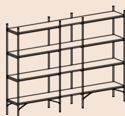
libreria media L225 medium shelving L225 225x38x165h
