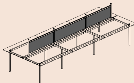
screen per bench 6 posti screen for 6-place workstation
