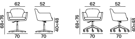
U174F02 Meeting Armchair Fixed Base U174F04 Meeting Armchair Base on Castors
