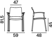
U178F00 U178F02 U178F04 Multiuse Chair Plastic Backrest and Seat
