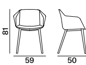
ST155F02 ST155F04 Community Chair Polypropylene Shell Plastic Legs or Wooden Legs
