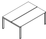
U559F646 120x123x72h U559F648 140x123x72h U559F650 160x123x72h U559F652 180x123x72h U559F654 200x123x72h
